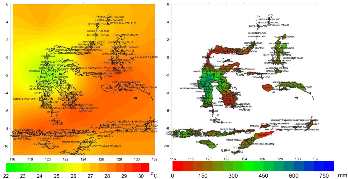
Figure 9.1: Temperature and Rainfall Projections for Wallacea
